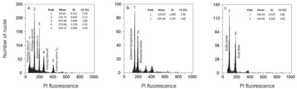
Fig. 1. Illustrative flow cytometric histograms of relative PI fluorescence intensity obtained after simultaneous analysis of nuclei isolated from the sampled taxa and the internal reference standard: (a) Pritzelago alpina with the occurrence of endoreduplication, and Raphanus sativus ; (b) Minuartia verna and Solanum lycopersicum ; (c) Scilla verna and Vicia faba . In each histogram, information of mean channel number (mean), DNA index (DI, defined as the ratio between the mean channel number of sample and reference standard) and coefficients of variation (CV, %) of each DNA peak are given. Please note the overall good quality of the histograms, as defined by the CV of each peak and by the low amount of background debris.
