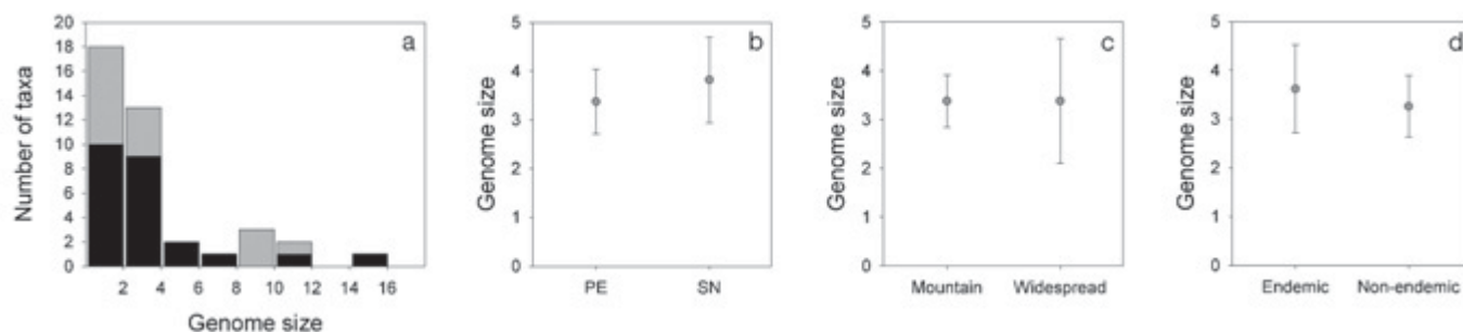
Fig. 2. Distribution of the genome size estimations among 39 high mountain taxa (a; black bars: Picos de Europa; grey bars: Sierra Nevada and comparisons of genome size variation (mean and SD, 2C/pg) between Picos de Europa (PE) and Sierra Nevada (SN) taxa (b), between plants specialized to live in mountain areas and those widely distributed (c), and between taxa endemic to restricted mountain ranges (Endemic) and not restricted (Non-endemic) (d).
