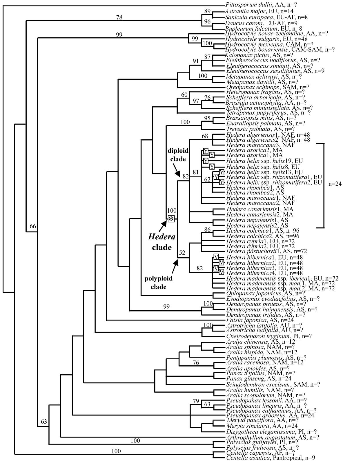
Fig. 3. Strict consensus tree of 115,800 most parsimonious trees of 1471 steps from the analysis of the 85 ITS sequences of the Araliaceae and Apiaceae (CI: 0.51; RI: 0.74). Pittosporum dallii served as the outgroup. Bootstrap values above 50% are shown above branches. Numbers after species names refer to population numbers as in Table 1, followed by distributional abbreviations (AA, Australasia; AF, Africa; AS, Asia; AU, Australia; CAM, Central America; EU, Europe; MA, Macaronesia; NAF, northern Africa; NAM, North America; PI, Pacific Islands; SAM, South America) and chromosome numbers, indicating a question mark (?) for cases of insufficient data.
