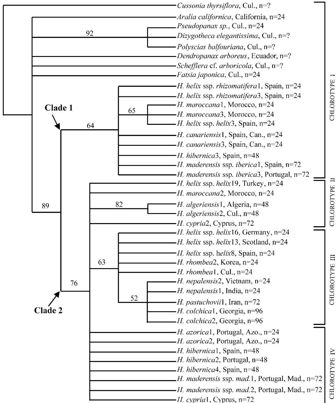
Fig. 4. Strict consensus tree of 114 trees of 73 steps (CI: 0.92; RI: 0.94) from the analysis of 41 trnT-L spacer sequences plus recoding of four indels, four affecting two sequences of the Araliaceae genera and two for the regions I and II of trnT-L (see text and Fig. 2). Cussonia thyrsoiflora served as the outgroup. Bootstrap values above 50% are shown above branches. Numbers after species names refer to population numbers as in Table 1 and Fig. 3, followed by country and region of origin, and gametic chromosome number. Abbreviations: Azo., the Azores; Can., the Canary Islands; Cul., cultivated and cultivars; Mad., Madeira; mad, maderensis. Accessions grouped by the four Araliaceae chlorotypes (cp. I, II, III, and IV).
