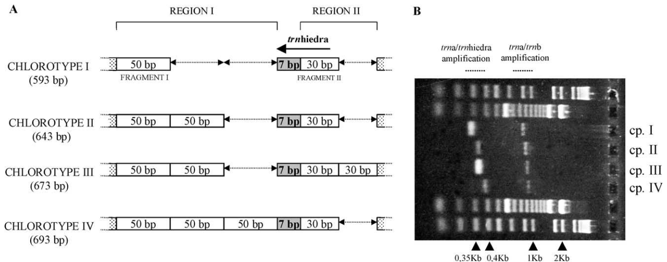
Fig. 2. Types of chloroplast (chlorotypes) of Hedera determined from different sizes of the trnT-L sequences. (A) Schematic representation of the four chlorotypes (cp. I, II, III, and IV), as aligned in the trnT-L sequence matrix. Region I has one, two, and three copies of a 50-bp fragment (fragment I); region II with one and two copies of a 30-bp fragment (fragment II). Relative position of the sites limiting the two regions and the new, reverse primer trnhiedra are indicated; (B) agarose gel resolution of the four chlorotypes from eight PCR amplicons when using primers trna/trnb (larger bands), and trna/trnhiedra (smaller bands) were loaded in four lanes: cp. I in H. maderensis spp. iberical1 ; cp. II in H. helix ssp. helix19 ; cp. III in H. colchical1 ; and cp. IV in H. hibernica2 .
