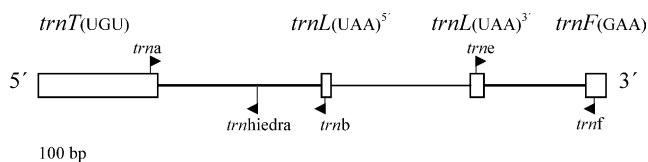
Fig. 1. Structure and directions of primers used to amplify trnT – L and trnL – F spacers. Proportional positions depicted for type I of chloroplast (chlrotype I) of Hedera (Taberlet et al., 1991). The internal primer trnhiedra was therein designed for amplification of a partial fragment of the trnT – L spacer.
